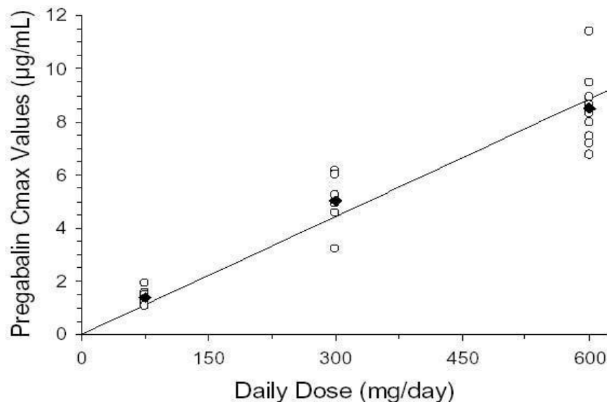
Figure 1. Individual and Mean Steady-State Pregabalin C max Values Following 75, 300 and 600 mg/day Given in Equally Divided Doses TID (q8h) to Healthy Volunteers a
